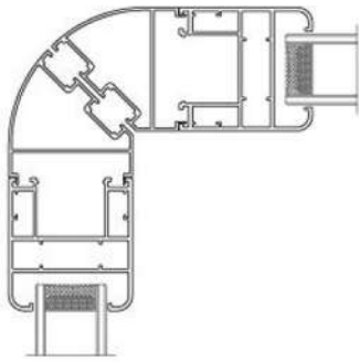
90° Corner Assembly Solution
